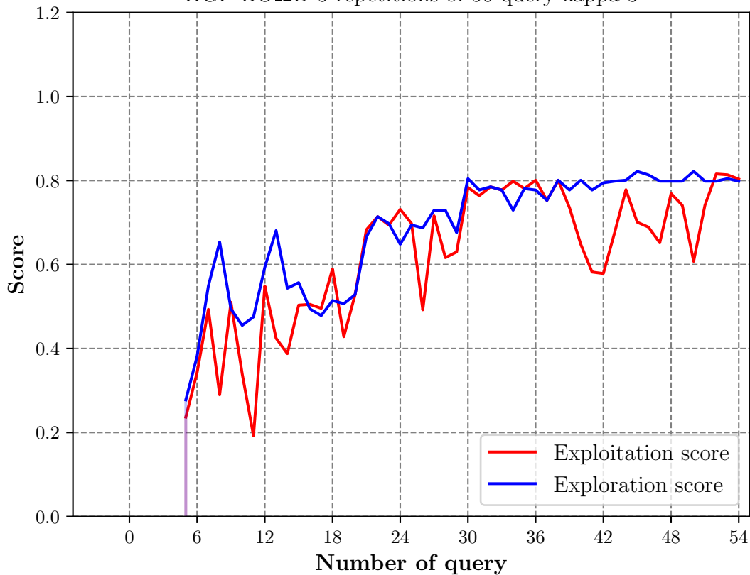
HGP-BO_2D 5 repetitions of 50 query kappa 3
